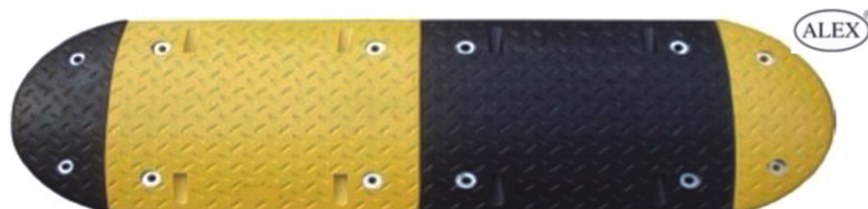
ALEX338 減速大路拱 Size: 500x430x50mm(中段) Size: 210x430x50mmH(端頭)
